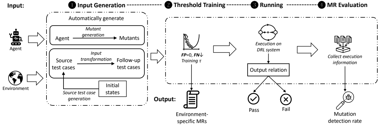
Figure 1. Logical workflow of MDPMORPH
