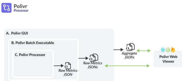
FIGURE 4. Layered architecture of Polivr Core. Each module outputs JSON files which are then uploaded and persisted to Polivr Web Viewer.
