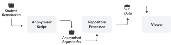
FIGURE 1. Conceptual pipeline diagram. Key modules are shown as shaded rectangles and are expanded upon in the following section. Modules are connected by generic data interchange representations.
