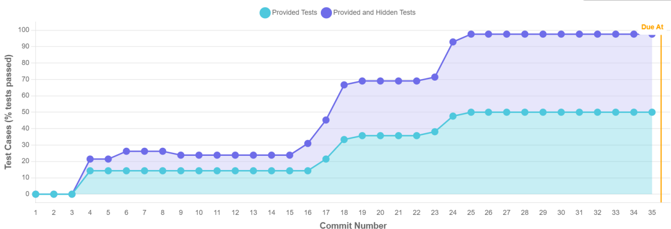
FIGURE 10. Line chart of the cumulative number of provided and hidden test cases passed for each commit in Repository 158. The student of this repository seems to make significant progress in test cases in commits 18 and 24. This suggests a consistent and gradual progression towards passing all test cases.
